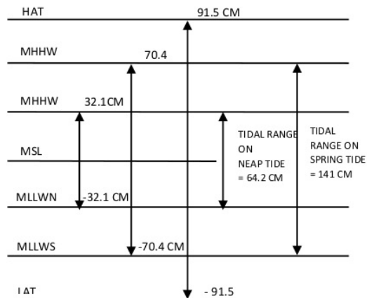
Figure 7. Tidal range in the research location
