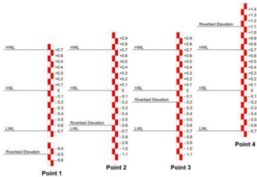
Figure 9. Tidal elevation at inspection points
