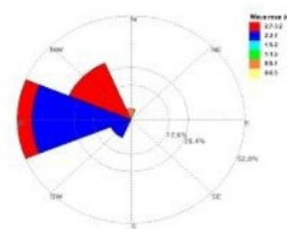
Figure 4. Wave rose diagram of the research location
