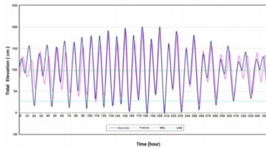
Figure 6. Water level elevation diagram in the research location
