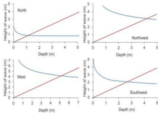
Figure 5. Breaking wave diagram in Jeneberang River Estuary from various directions
